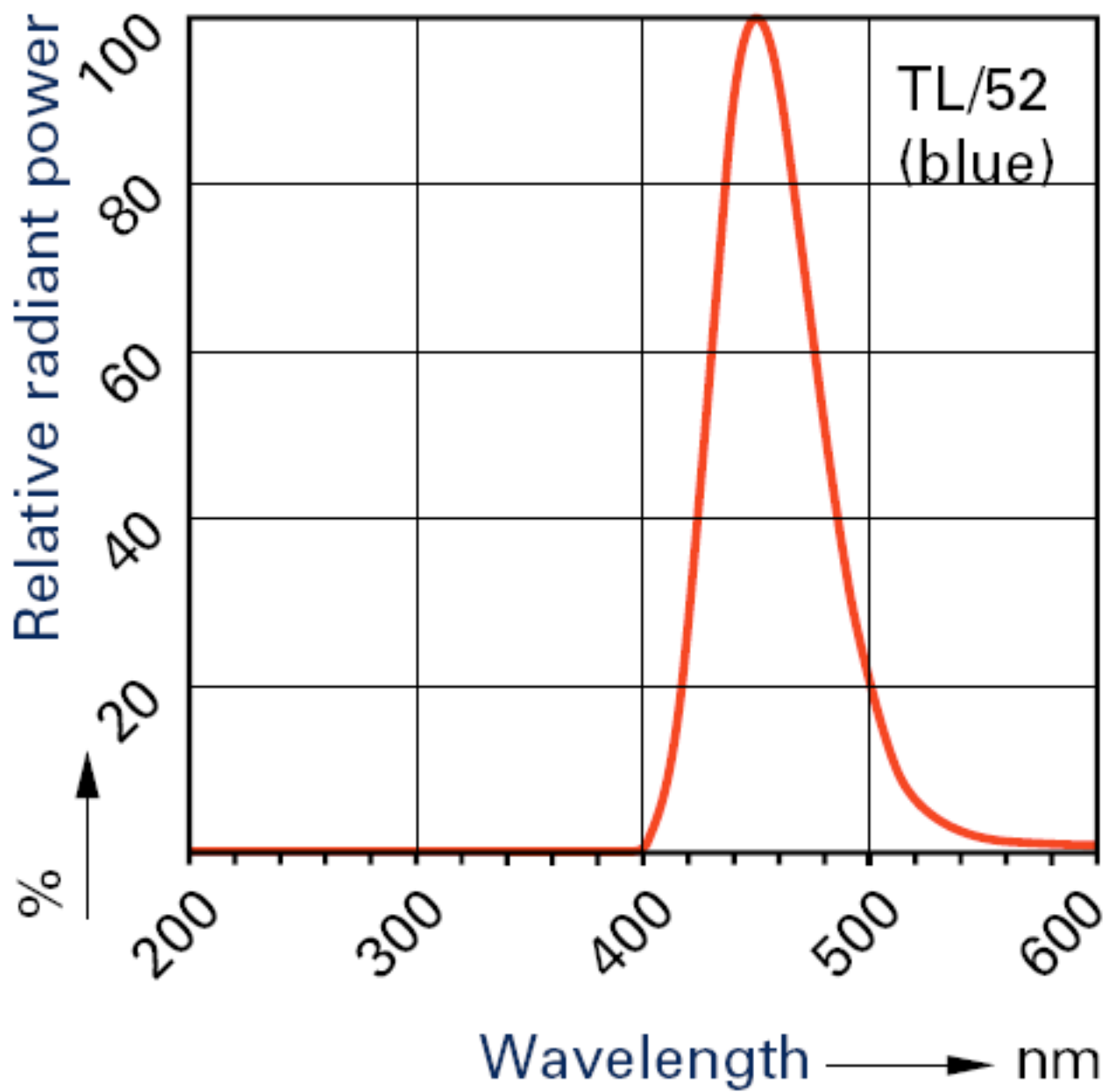
Spectrum of a blue lamp TL/52: emission peak at wavelength of 450 nm.
